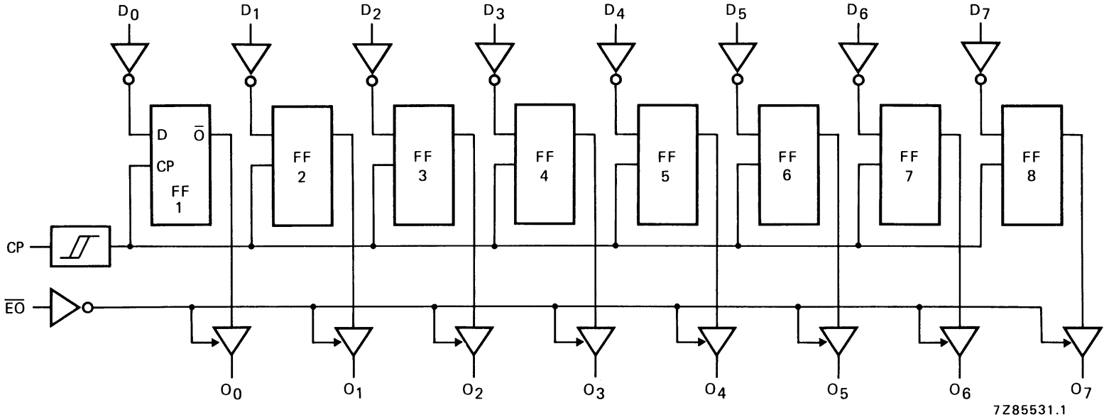
Fig.3 Logic diagram.
